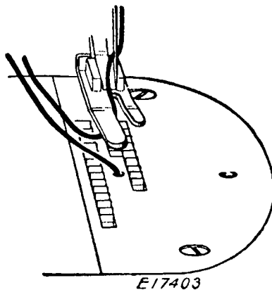
FIG. 15 THREADS IN POSITION TO COMMENCE SEWING
