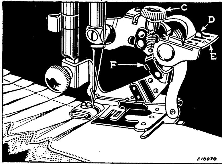
FIG. 69. PLAITING WITH THE RUFFLER
