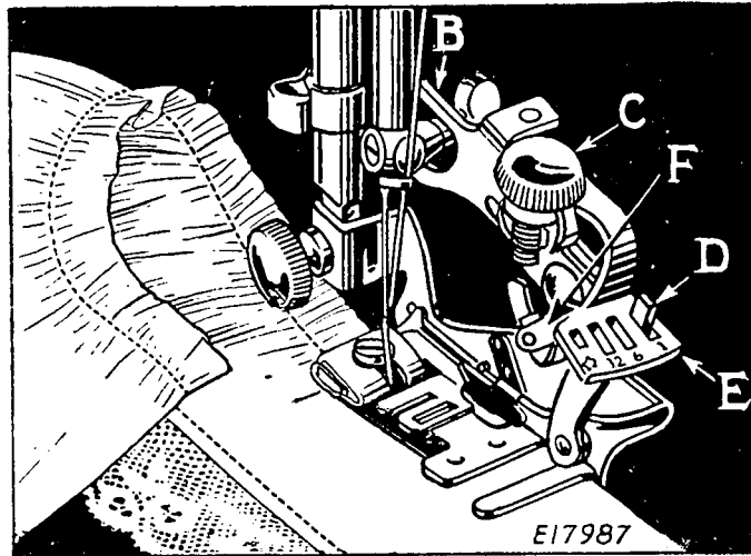
FIG. 61. GATHERING WITH THE RUFFLER
