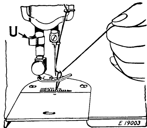
FIG. 14 DRAWING UP THE BOBBIN THREAD
