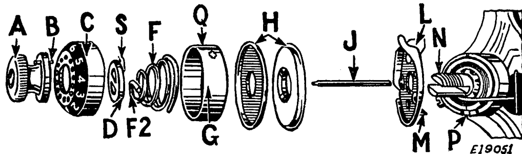
FIG. 22. NEEDLE THREAD TENSION DISASSEMBLED
