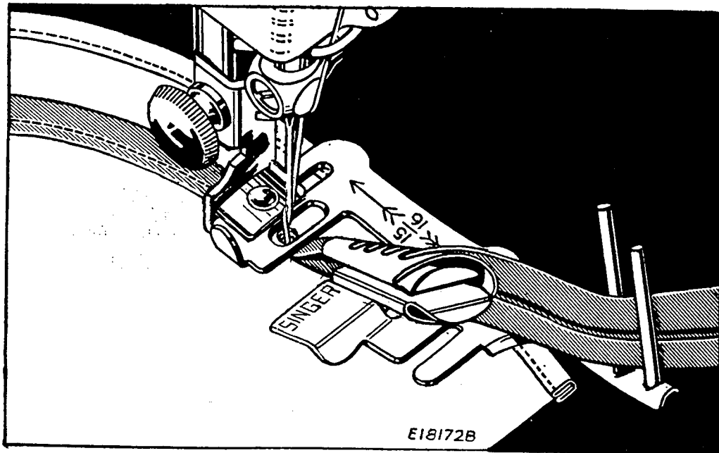
FIG. 50. APPLYING A FRENCH FOLD
