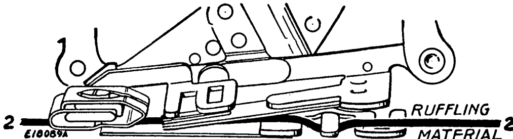
FIG. 72. CORRECT POSITION FOR THE MATERIAL
