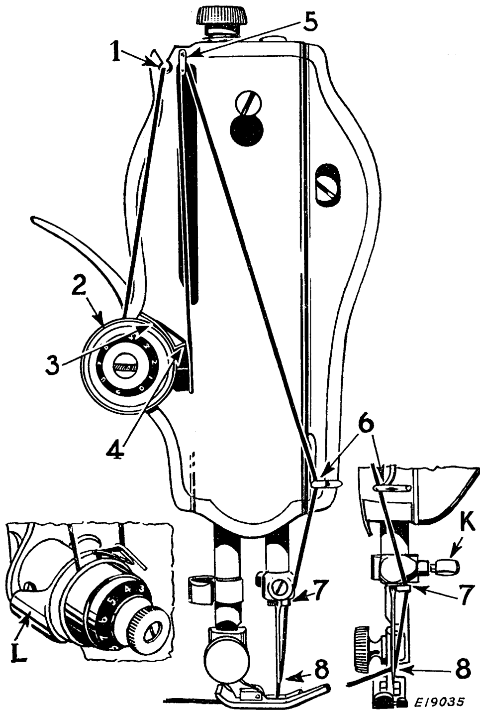
FIG. 6. UPPER THREADING
