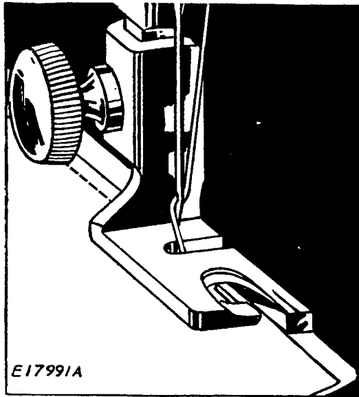
FIG. 39. MAKING A FELLED SEAM (FIRST OPERATION)
